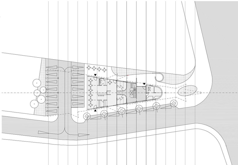
Ground-floor plan
