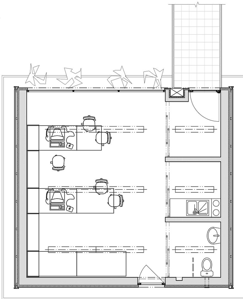
Ground plan
