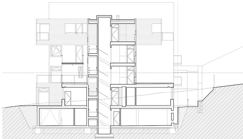
Cross-section object A
