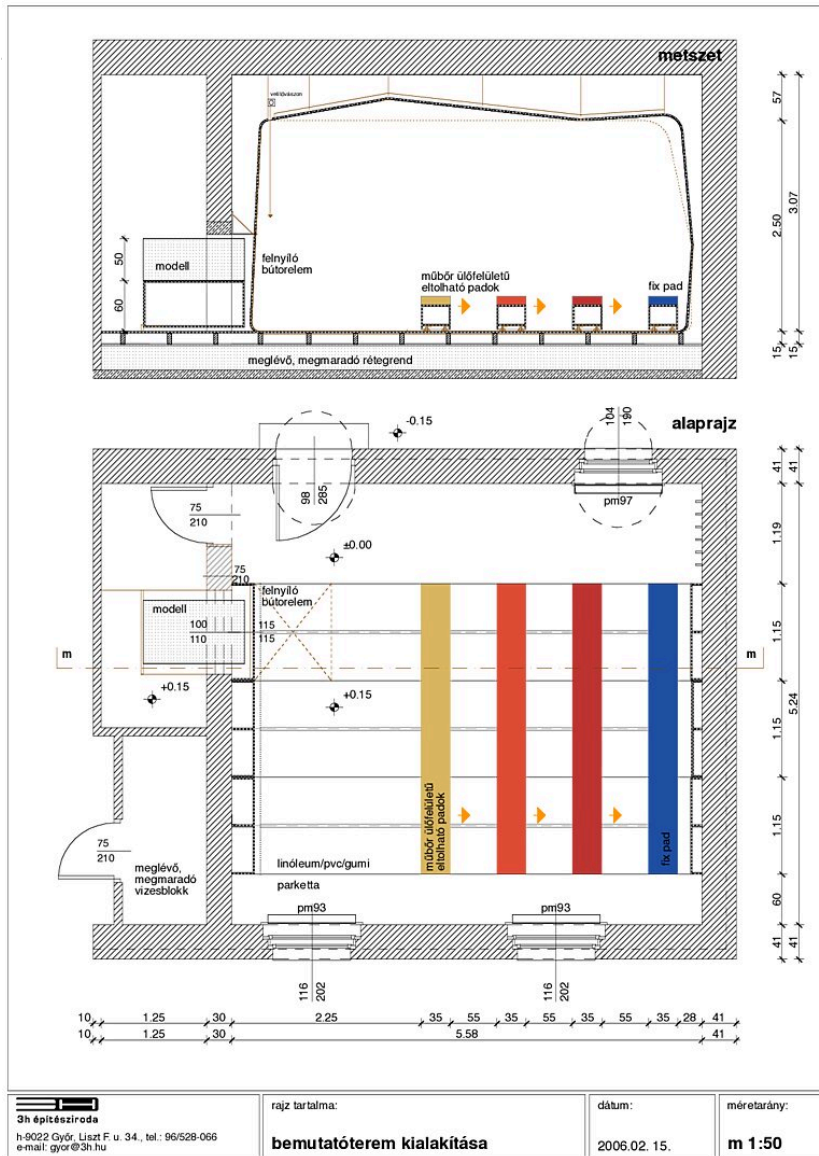
floor plan, section
