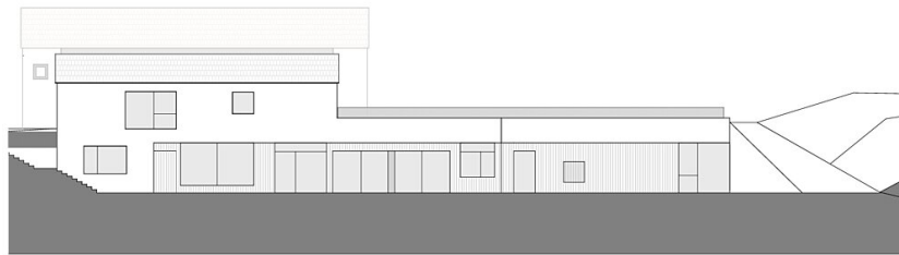
WESTFASSADE 1 2 5 10m
