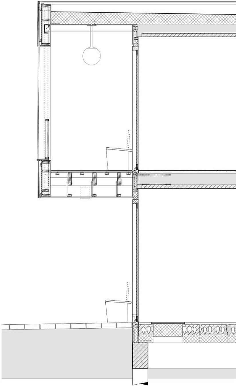
Section veranda
