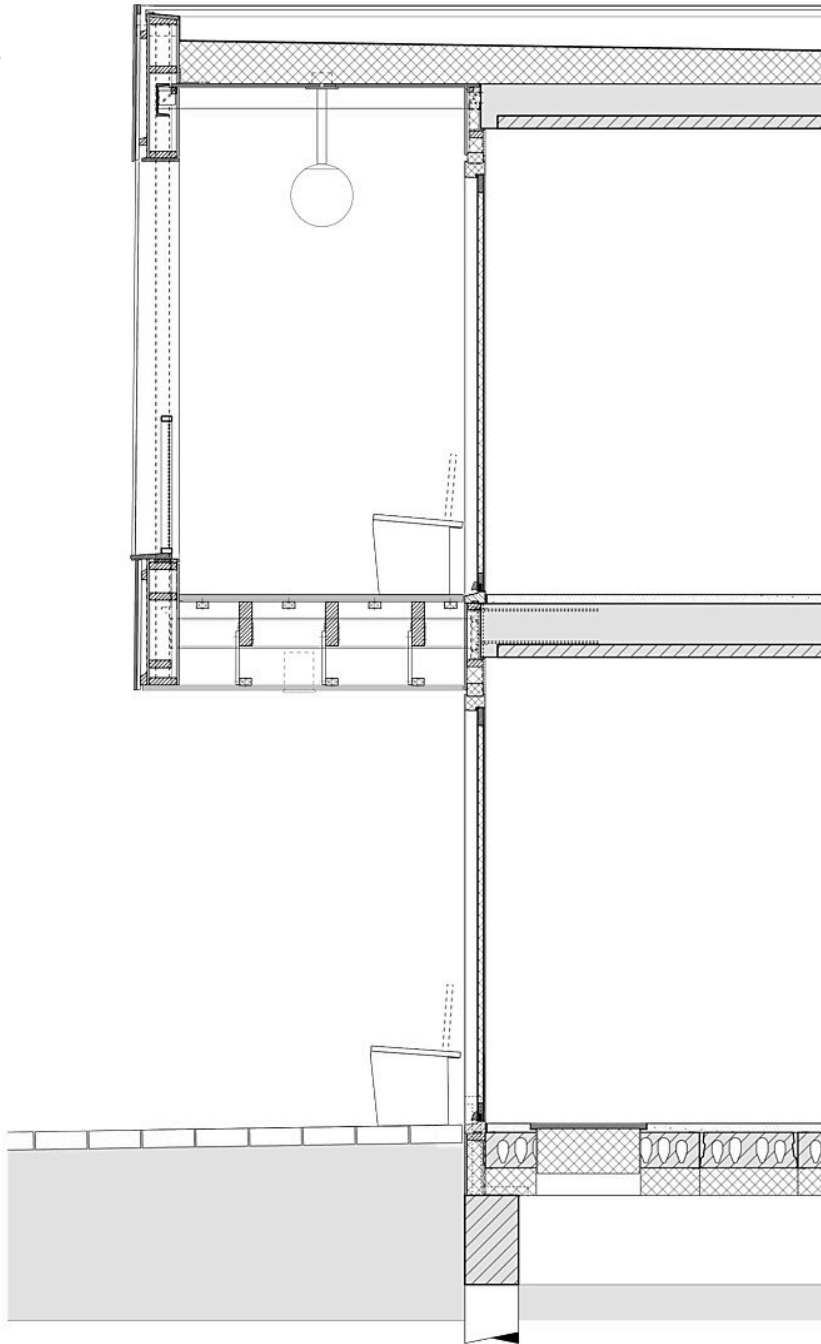
Section veranda
