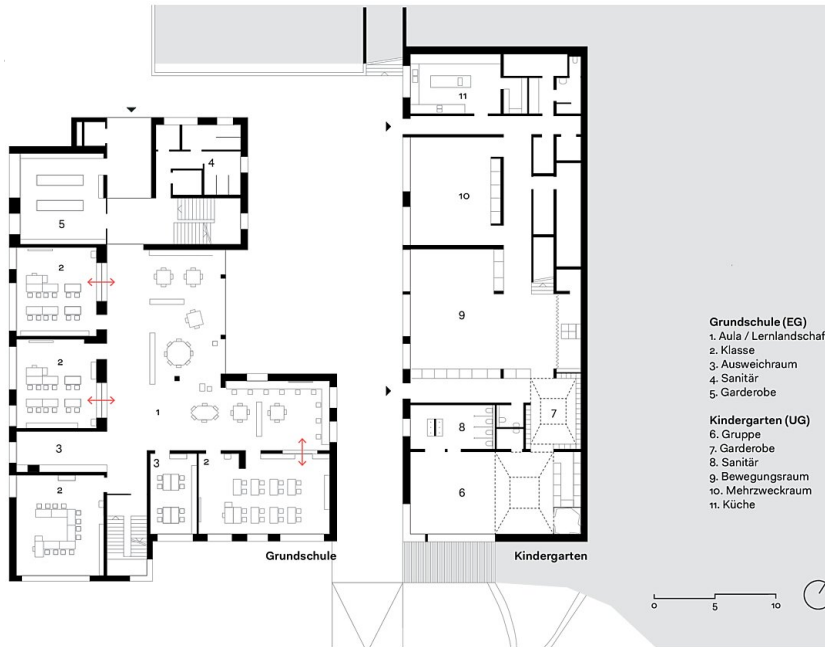
Grundriss EG-UG
