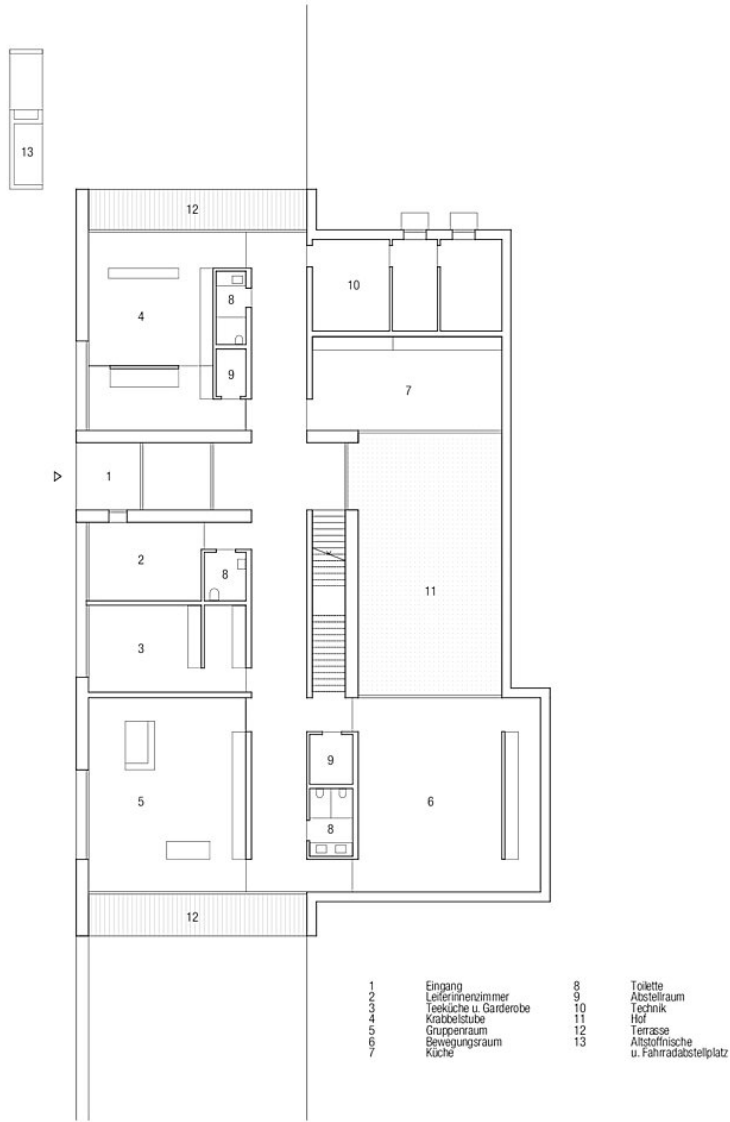
Grundriss EG :200
