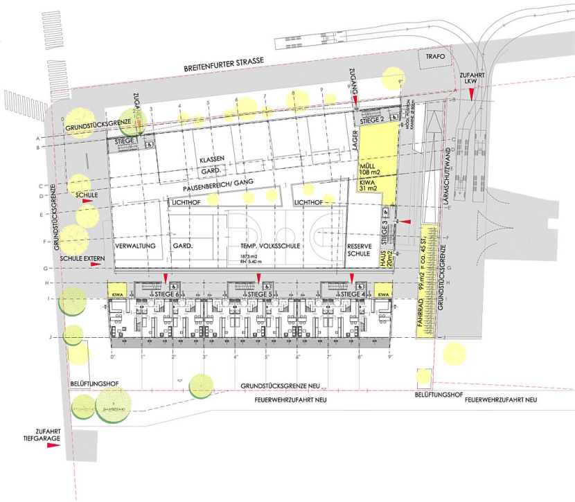
EG Detail
