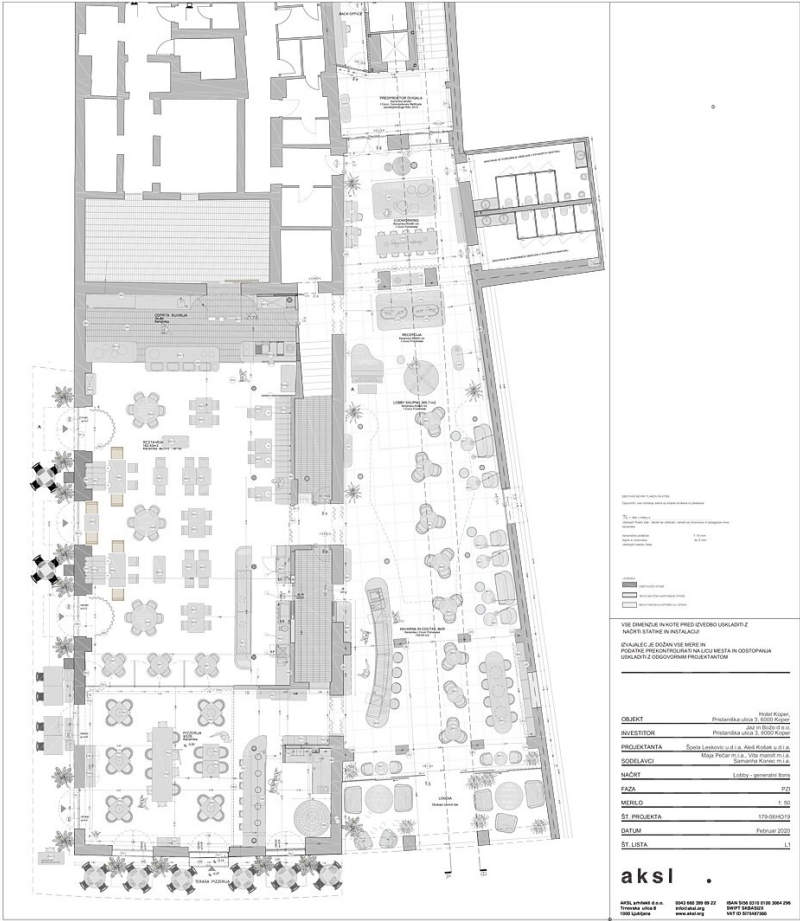
Lobby, Restaurant, Pizzeria
