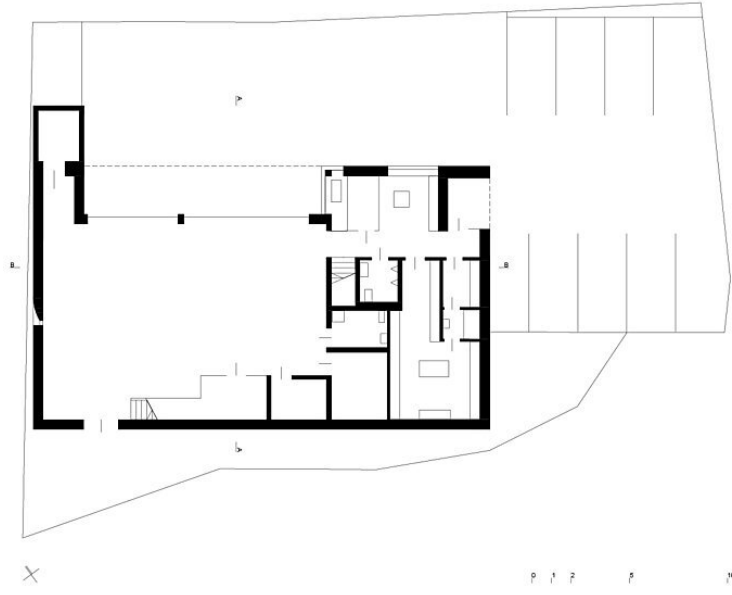
Grundriss EG 1_200
